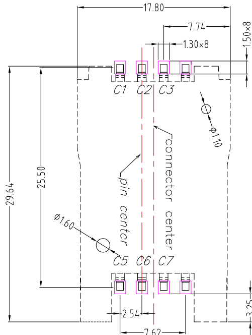
PCB LAYOYT
