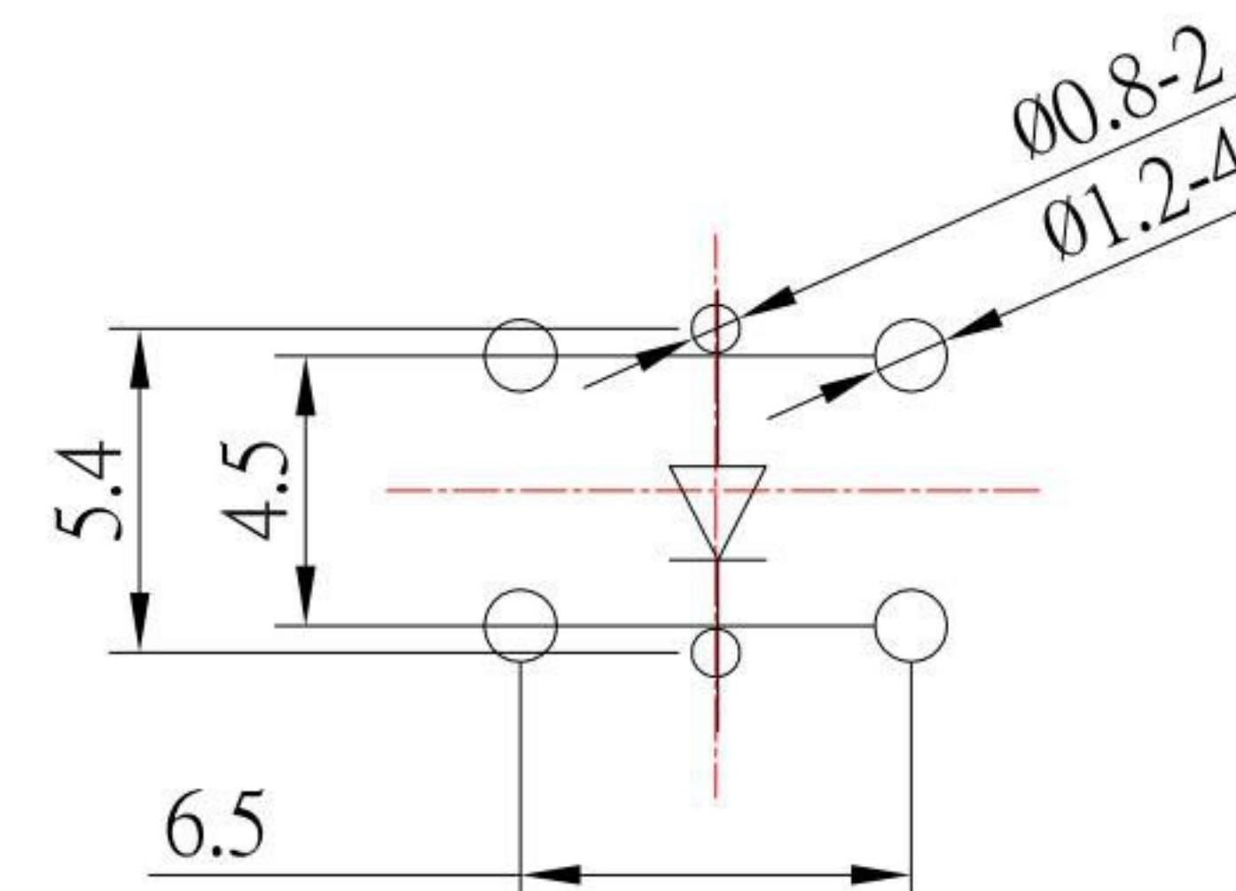
MOUNTING PATTERN
