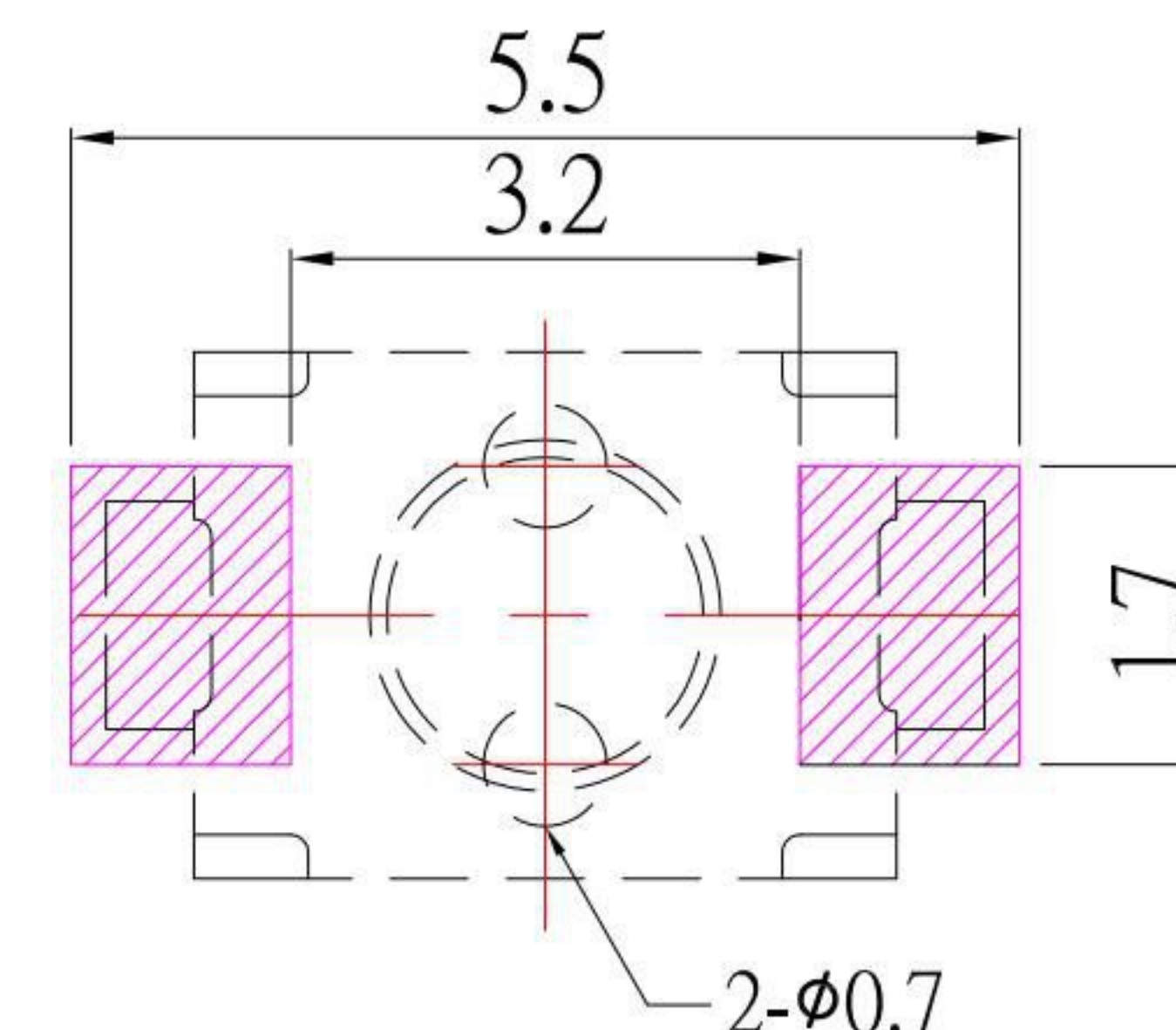
P.C.B. LAYOUT MOUNTING PATTERN
