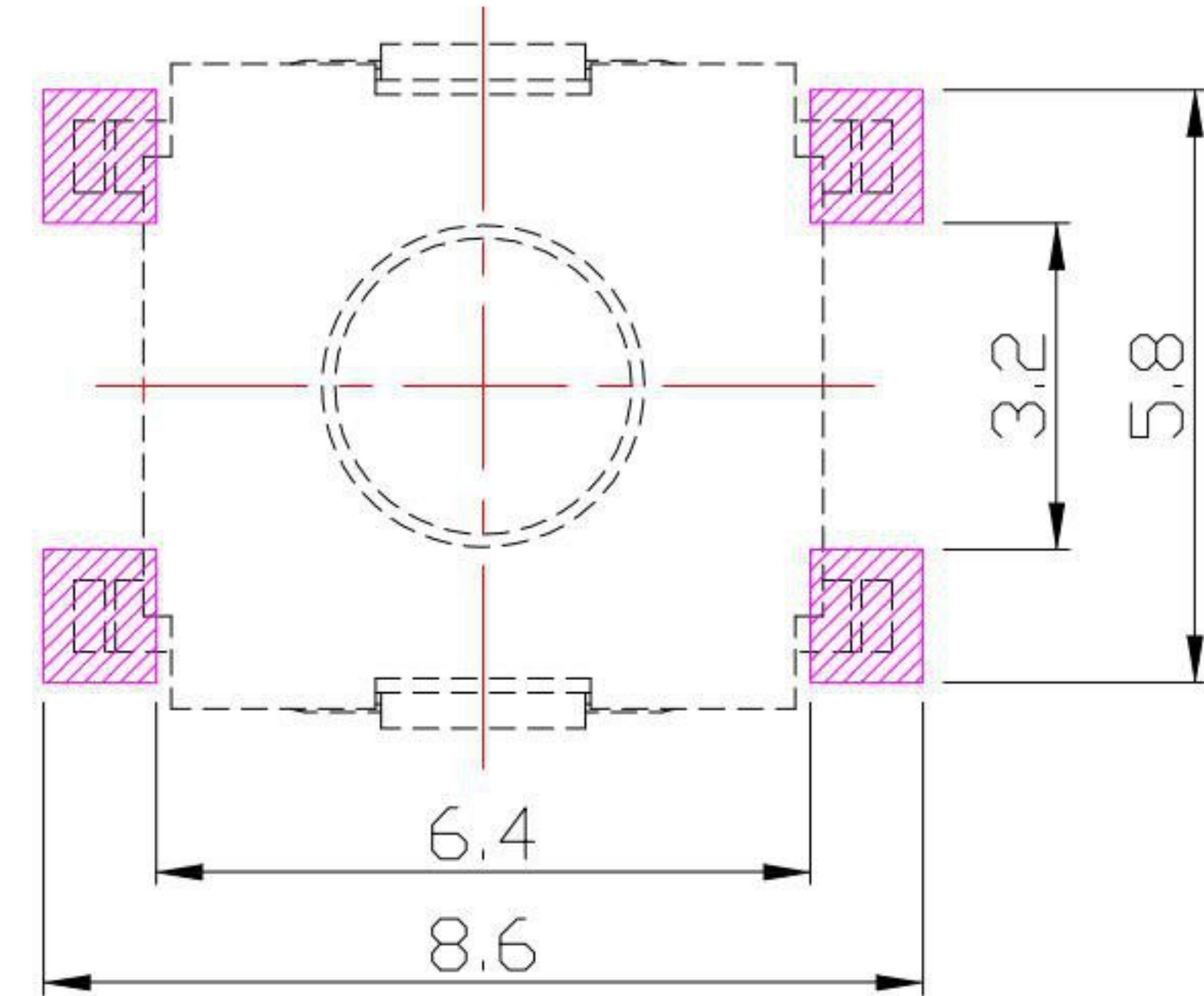
P.C.B MOUNTING PATTERN DIMENSION
