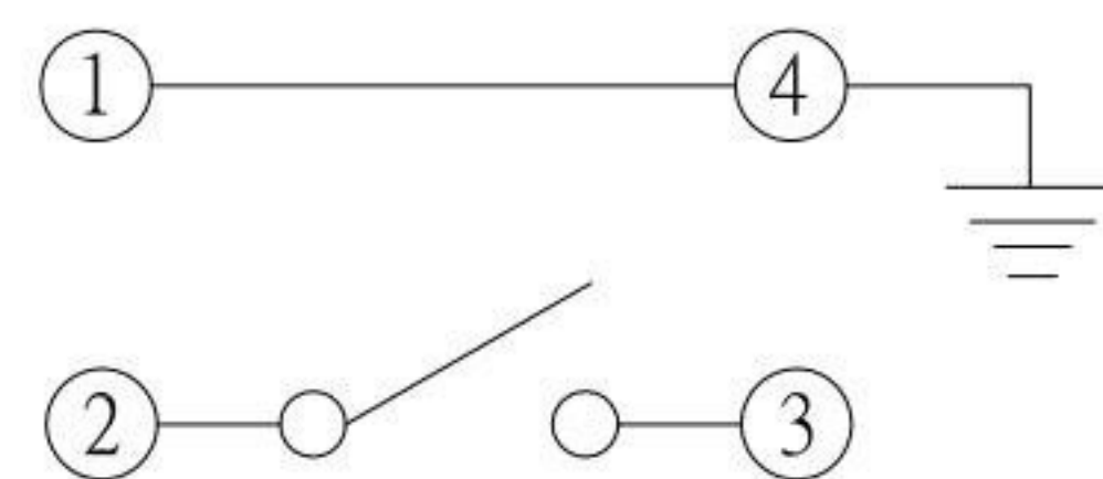
CIRCUIT DIAGRAM
