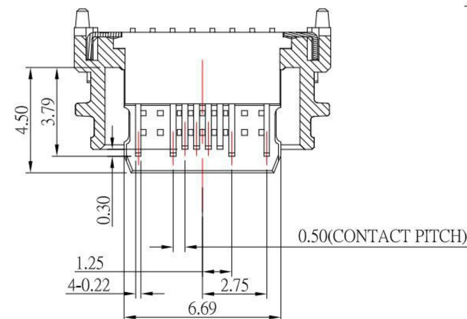
SECTION B-B
