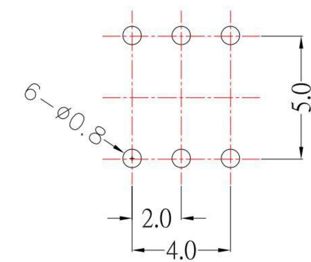
P.C.B MOUNTING PATTERN
