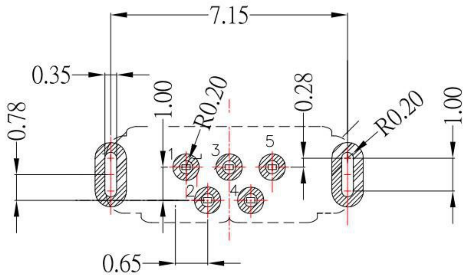
P.C.B LAYOUT MOUNTING PATTERN
