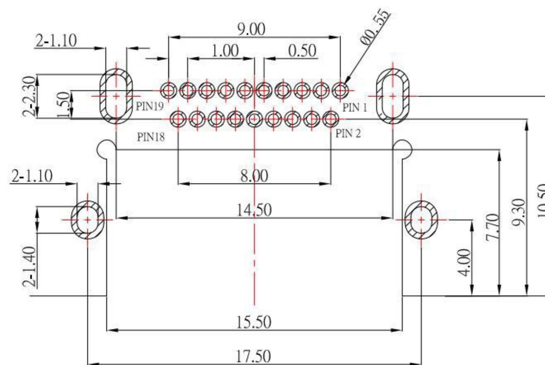
RECOMMENDED PCB LAYOUT(TOP VIEW)
