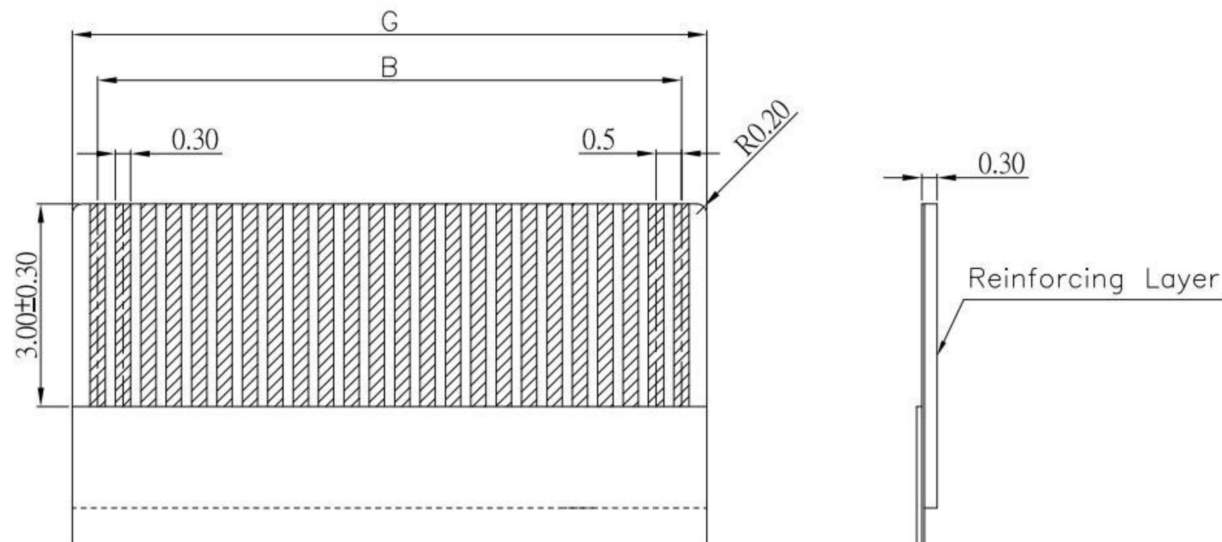
APPLICABLE FPC/FFC
