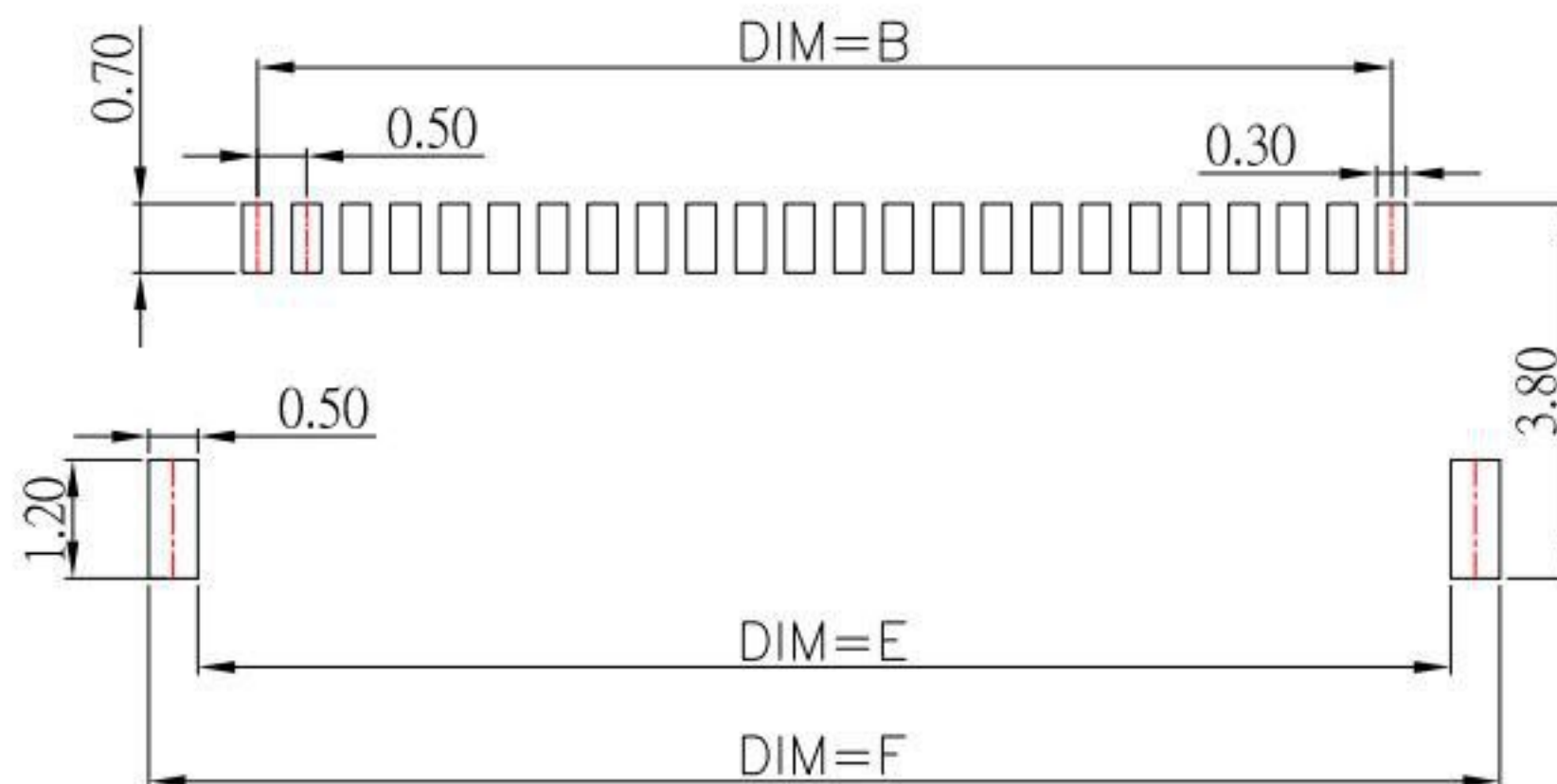
PCB LAYOUT
