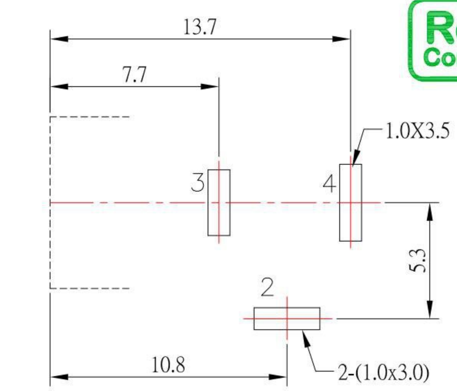
P.C.B LAYOUT MOUNTING PATTERN (TOP-VIEW)
