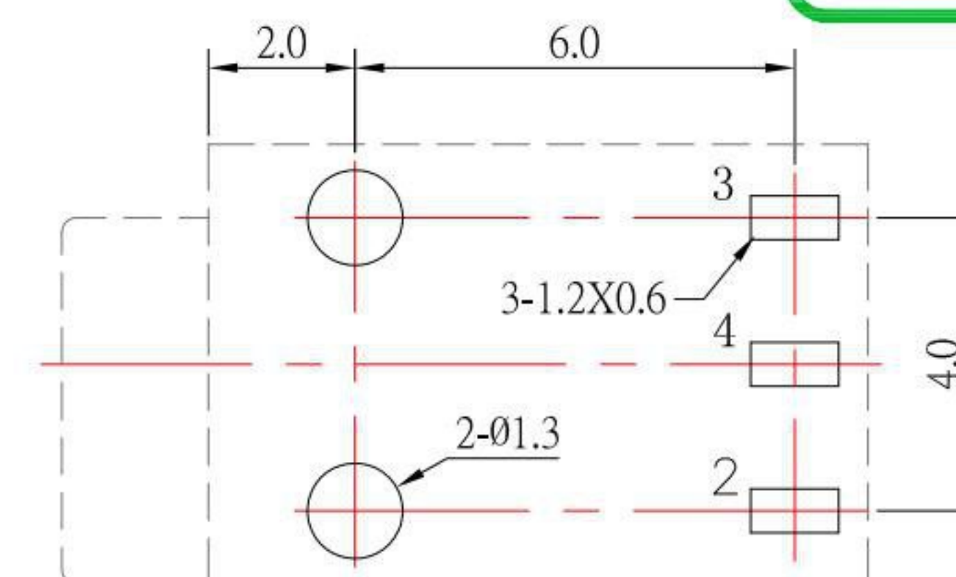
P.C.B LAYOUT MOUNTING PATTERN (TOP VIEW)
